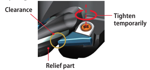
Fig.2 Install inserts
